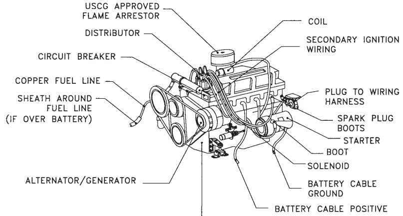
DIAGRAM 2 Inboard and Sterndrive Runabout
