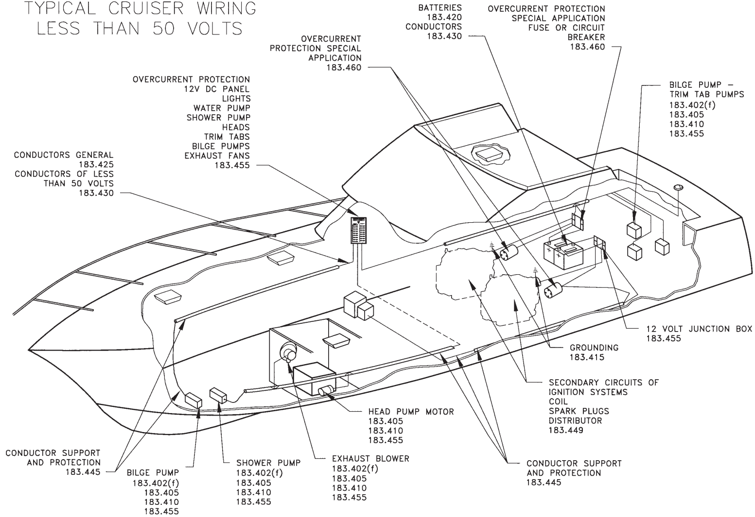
DIAGRAM 5 Cruiser — Wiring — Less Than 50 Volts
