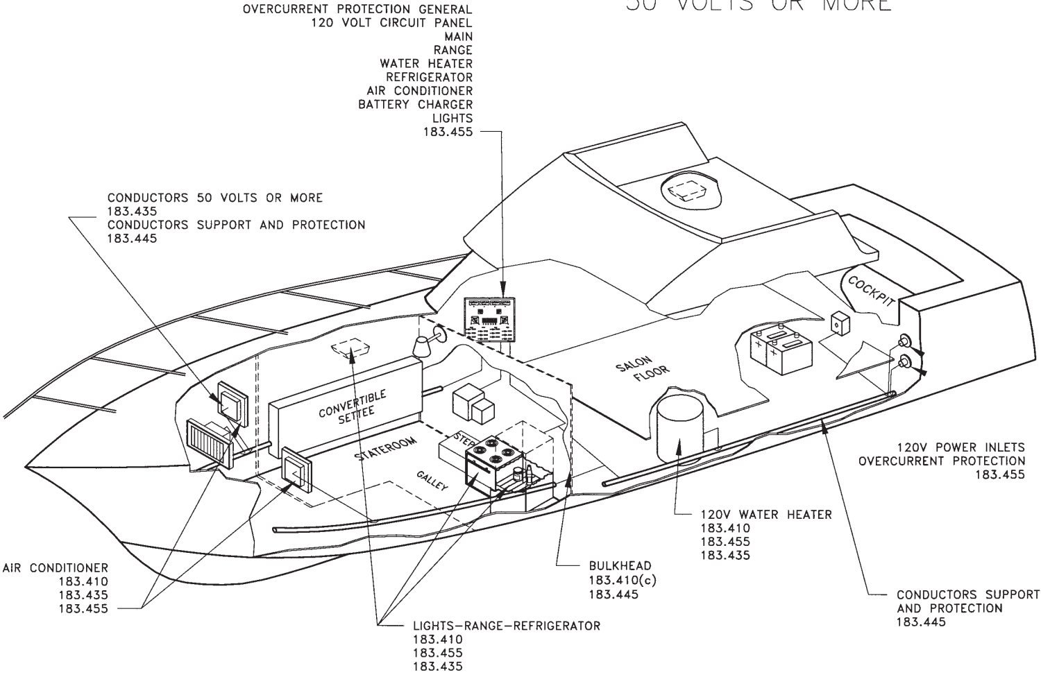
DIAGRAM 6 Cruiser — Wiring — 50 Volts or More
